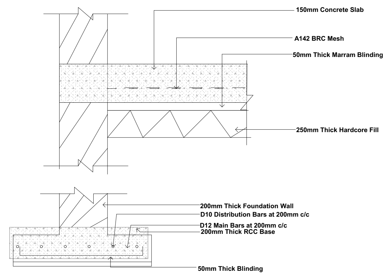
FOUNDATION DETAIL
